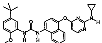
1-(5-tert-Butyl-2-methoxy-phenyl)-3-[4-(2-cyclopropylamino-pyrimidin-4-yloxy)-naphthalen-1-yl]-urea;
